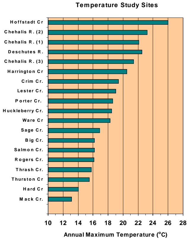
Figure 3.1 Annual warmest temperature at the 19 temperature study sites included in the temperature risk assessment.
