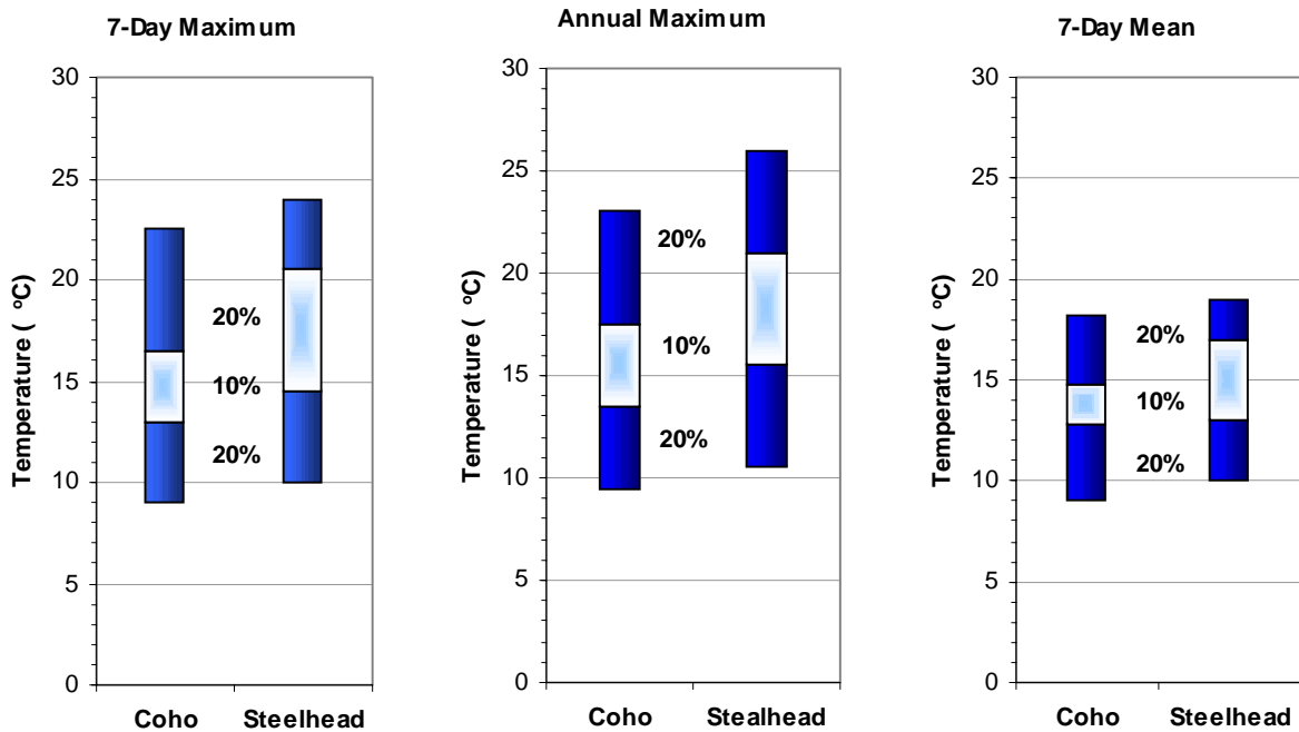
Figure 6.8 Ranges of temperature where reduction from maximum growth is 0-10% and 11-20%. At temperatures above and below these ranges RMG exceeds 20%.
