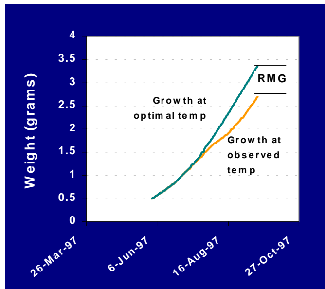
Figure 6.3 Illustration of the reduction in maximum growth based on two temperature scenarios; growth at constant optimal temperature and with the variable growth rate based on the site's temperature regime.
