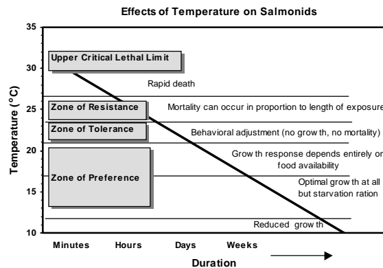
Figure 8.1 The general biological effects of temperature on salmonids. Effects depend on the level of temperature and its duration. Two important elements of temperature affect the growth and survival of fish: 1) the relationship between temperature, metabolism and food conversion efficiency as it controls growth over relatively long periods, and 2) the thermal tolerance of fish to lethal temperatures over relatively short periods. Fish have various physiological and behavioral mechanisms that enable them to resist adverse effects of temporary excursions into temperatures outside of their preferred or optimal growth range but within the upper critical lethal limit.
