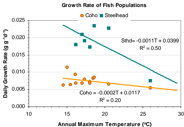
Figure 5.12 Growth rate calculated by the model averaged for the sampling period in relation to annual maximum temperature at each site.
