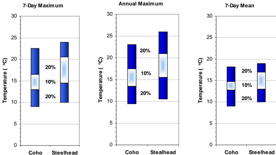
Figure 7.1 Range of temperature where reduction from maximum potential growth (RMG, %) was 10 and 20% during the summer months for coho and steelhead, using three temperature indices. (See Section 6 for methods and Table 6.2 for results by site. RMG is greater than 20% at temperatures outside of the temperature ranges indicated. RMG is minimized near the optimal temperature for each species and increases at temperatures warmer or cooler than the optimal.
