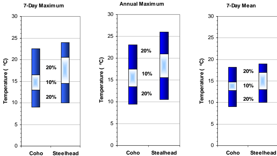
Figure 8.4 Temperature range for increments of growth loss associated with long-term temperature regime as expressed for 3 temperature indices and 2 species of salmonids. The inner range represents up to 10% growth loss and the outer range represents up to 20% growth loss. Above and below the ranges shown the growth loss exceeds 20% and was as high as 50% near the extremes of the temperature range. Risk assessment associated with growth loss suggests that a 10% limit would prevent any measurable effect on average coho population weight. A loss of 20% would be detectable and the temperature associated with this level of growth loss coincides with temperatures associated with avoidance behavior. Therefore, thresholds selected at 10% may be most appropriate for establishing temperature criteria. The threshold temperature varies with each index.
