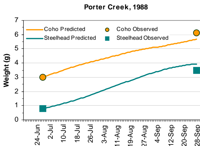
Figure 5.10 Weight prediction and observed fish weights for coho and steelhead populations at Porter Creek, 1988.
