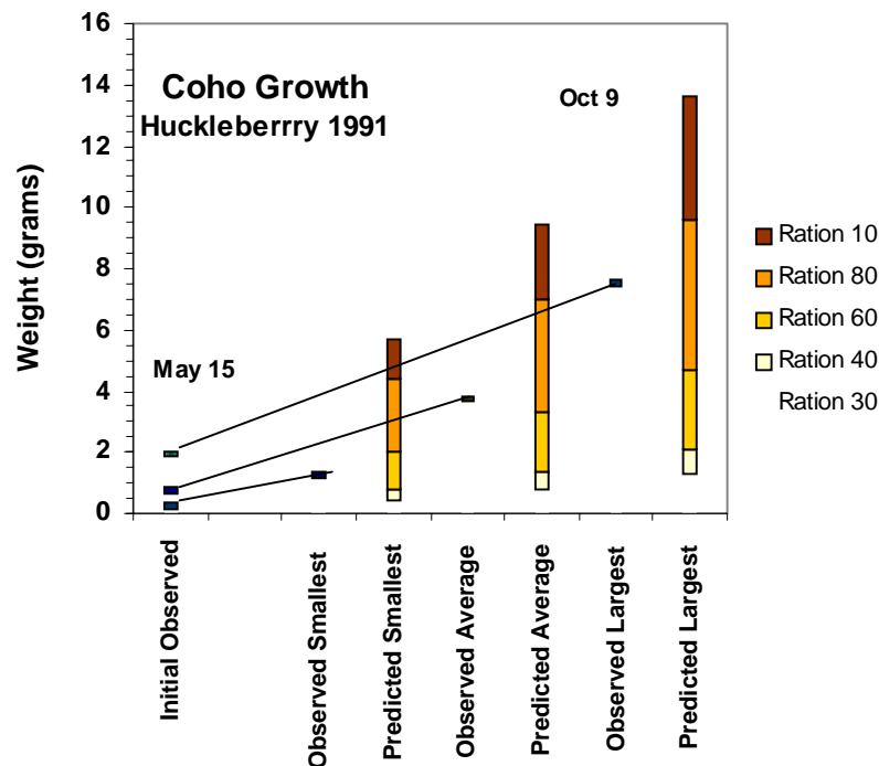
Figure 5.14 Observed and predicted weight of coho in Huckleberry Creek (1991). The growth of the smallest, average, and largest fish at the start of the summer (May 15) were modeled for the full range of satiation (shown in bars). Weight of each class at the end of the period (Oct 9) are shown at the end of the summer relative to growth simulations.
