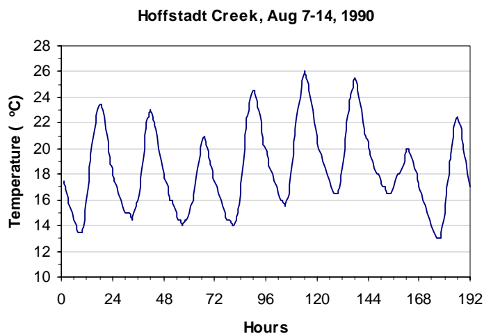
Figure 4.4 Hourly temperature during the warmest 7-day period at Hoffstadt Creek in 1990.
