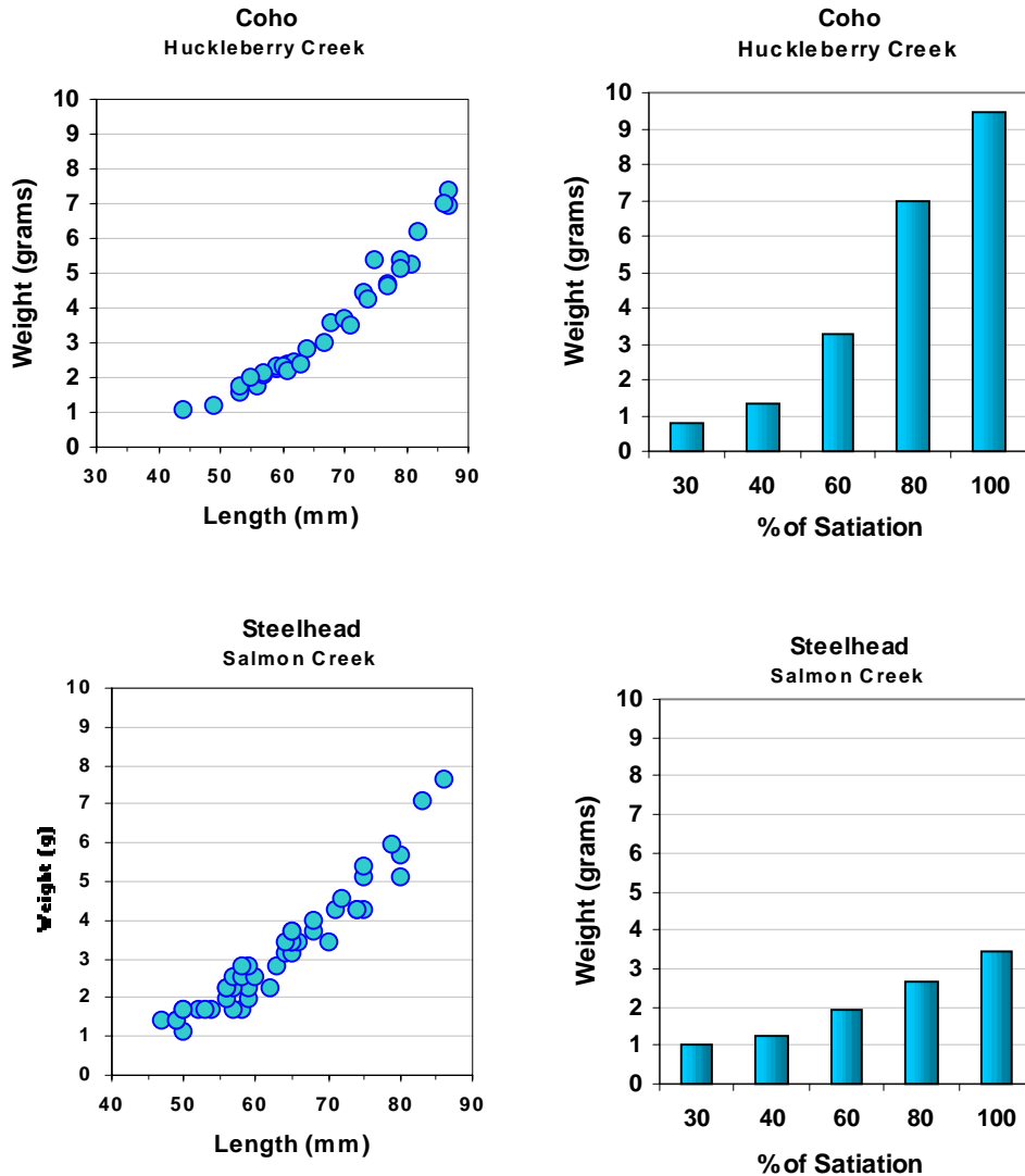
Figure 5.13. Examples of length-weight relationships for coho salmon population at the end of summer growing season at Huckleberry Creek and the steelhead trout population at Salmon Creek. Also shown are the predicted weight for each ration for Huckleberry Creek and Salmon Creek, calculated with the site's temperature from the period between population sampling, and a starting weight as observed at the site at the initial sampling.
