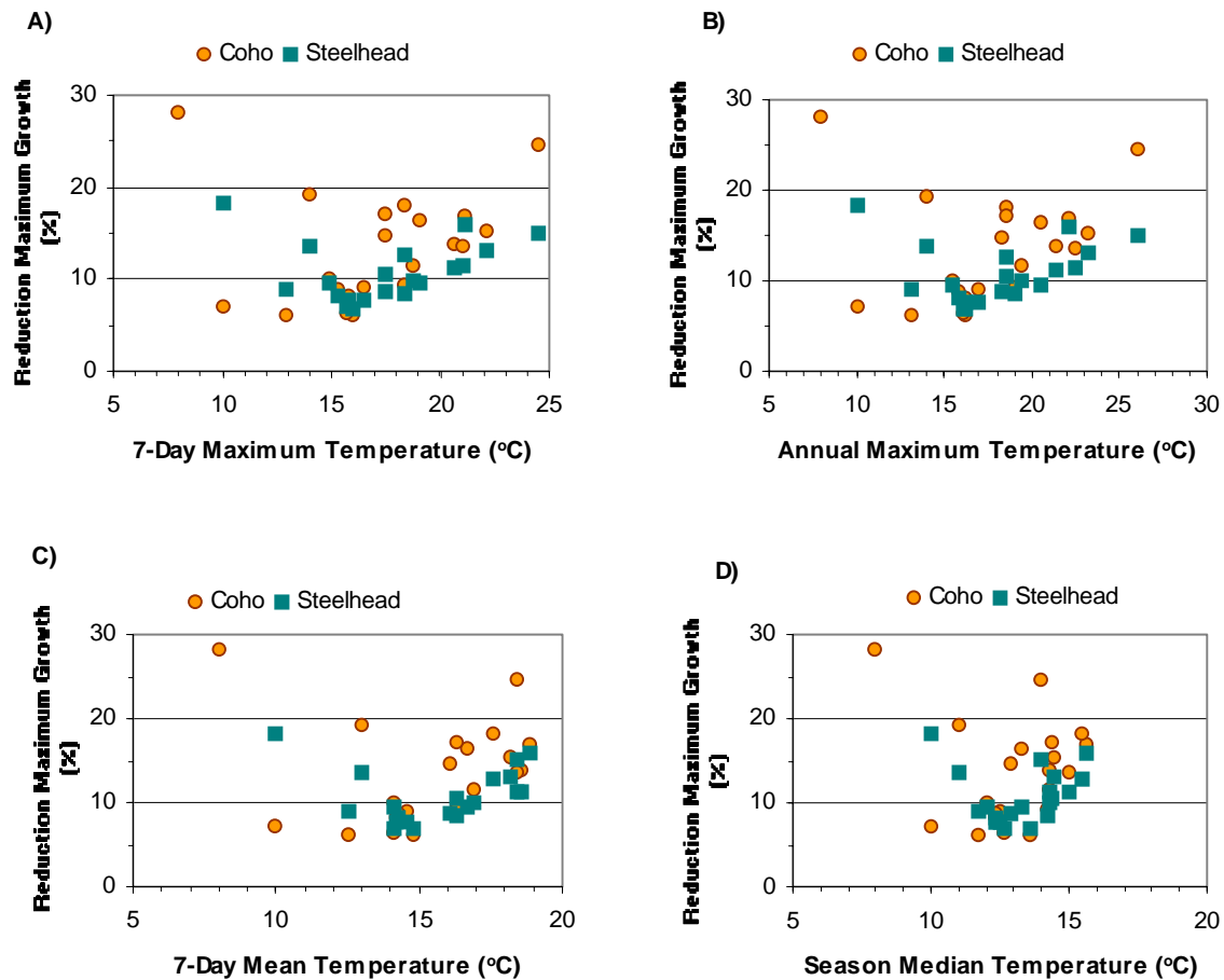
Figure 6.4 Estimated growth risk at temperature study sites in relation to several time-averaged temperature metrics: A) 7-day maximum, B) annual maximum, C) 7-day mean, and D) median temperature for the simulation period.
