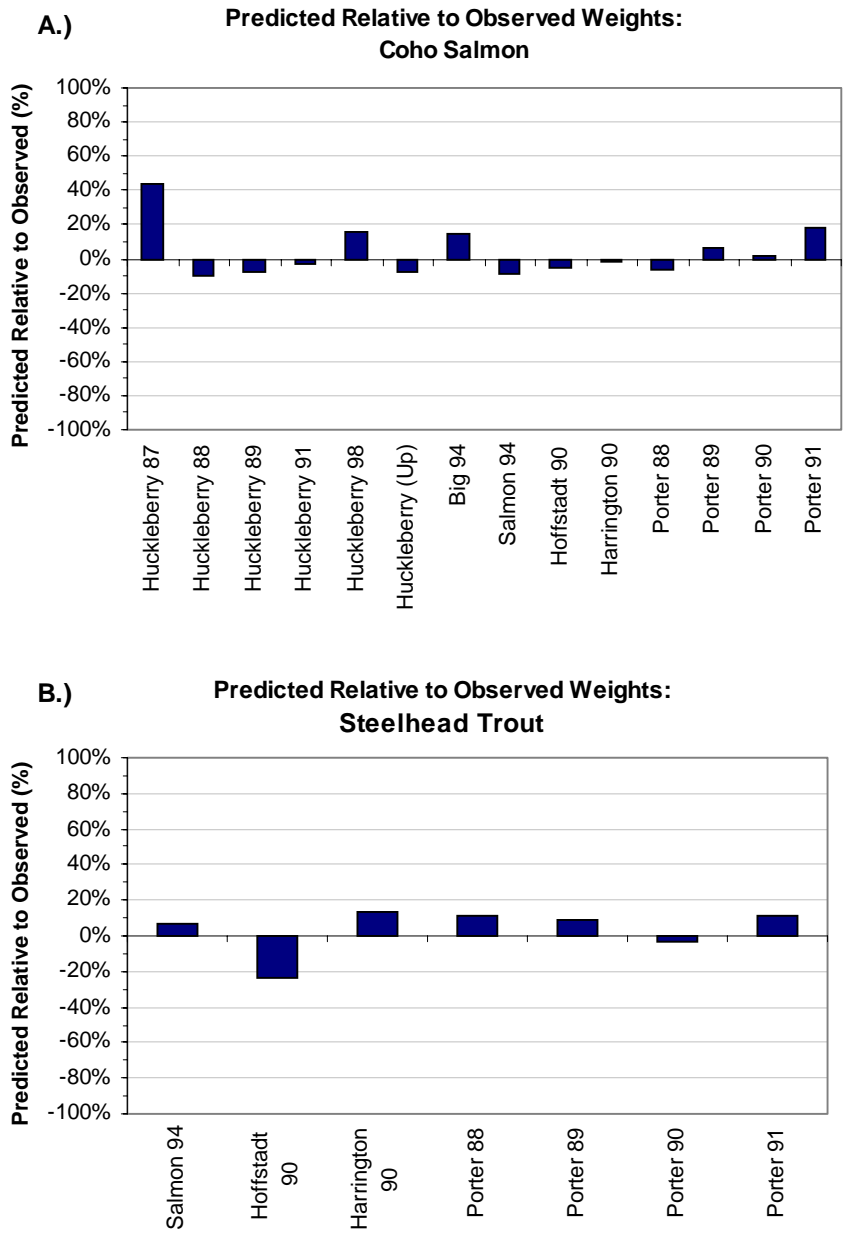
Figure 5.11. Differences between predicted and observed average weights of fish populations.
