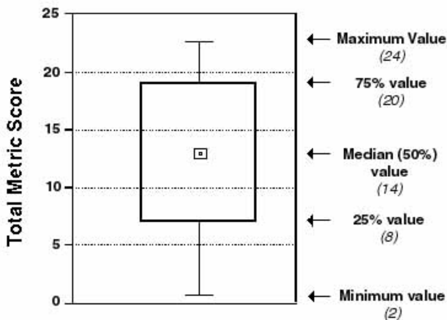
Figure 6.4 Example of a box plot
