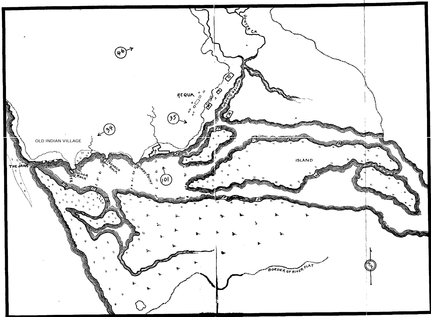
Fig. 9. Low-tide map of Klamath Estuary, 1920. River depths recorded in feet.
