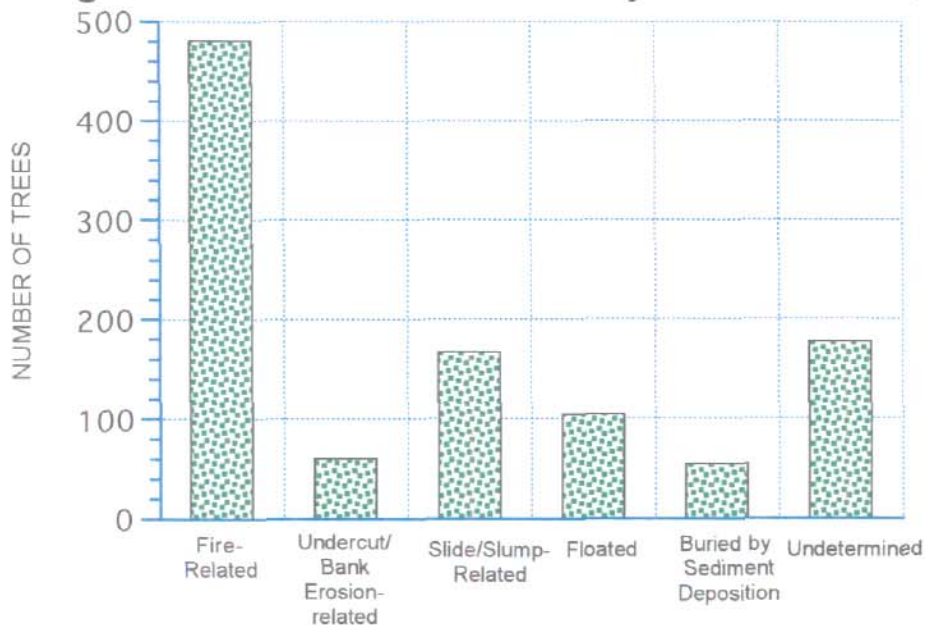
Figure 5. A) The amount of woody debris before and after fire is shown. Of the 1,043 woody debris elements influencing the channel, 86% are alders. The amount of slumps and debris jams are also shown for the second two years. B) The way that woody debris is recruited to the channel is shown. For wood listed as floated, its method of recruitment could not be determined.
